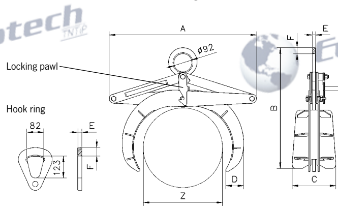
Model TRU, hook ring for grabs for 2000 kg and up capacity. Locking pawl locks open grab in place.
