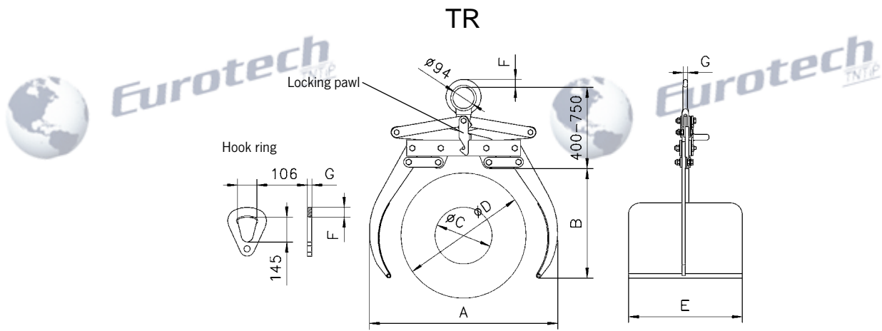
Model TR, hook ring for grabs for 2000 kg and above. Locking pawl keeps the grab in the open position.
