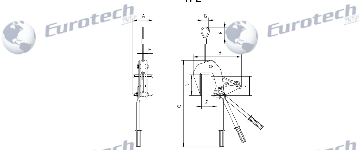
Model TPZ, up to 400 kg equipped with rope, from 750 kg equipped with chain.
